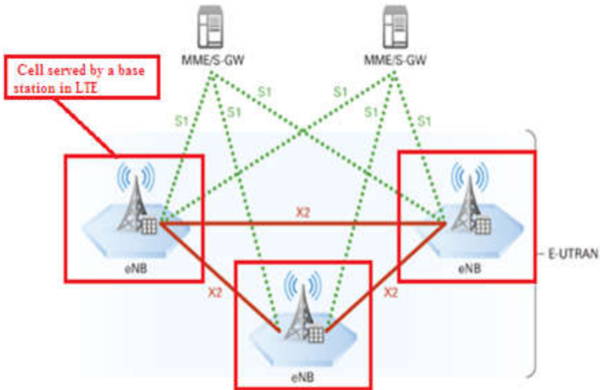
Figure 2: E-UTRAN Architecture
