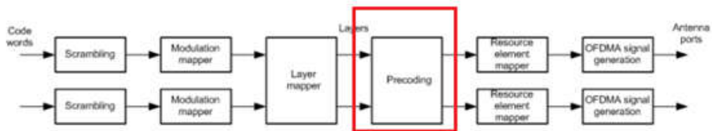
Figure 12: LTE downlink
