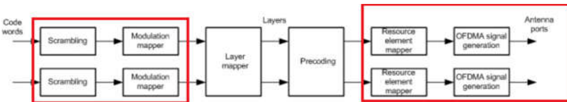
Figure 12: LTE downlink
